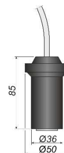
Figur 8. GA-SG1-sensor
